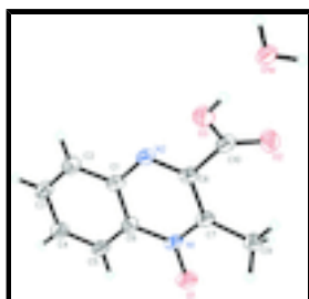
Fig. 1. The molecular structure of the title compound, showing the labelling scheme. Displacement ellipsoids are drawn at the 30% probability level for all non-H atoms.
