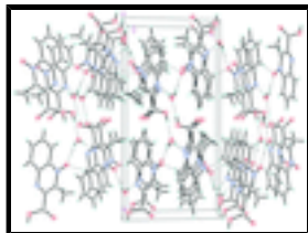
Fig. 2. Part of the crystal structure of the title compound viewed along the a axis. Hydrogen bonds are shown as dashed lines.
